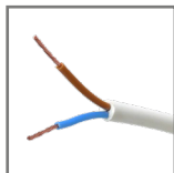
cable with poly-vinyl chloride insulation (H05VV-F) 2 x 1.0 mm 2
