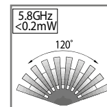
MS – built-in microwave sensor detection range: 120° max.7m time: 20 s illuminance < 20 lux
