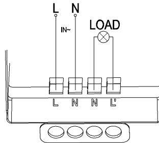
L - live wire; N - neutral wire supply and neutral load (eg. housing); L' – live wire load (eg. housing)
