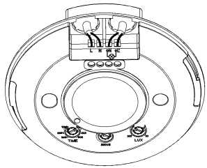
The wires come in and out from the bottom
