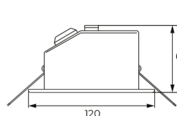
TLR2-3ZS-AT3H
