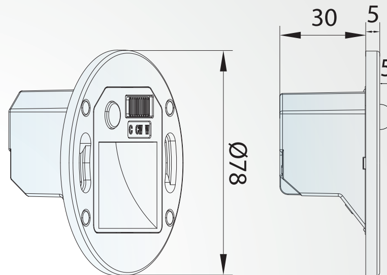
OST-001WH-CCT-PIR OST-001WH-CCT-PIR-MSV
