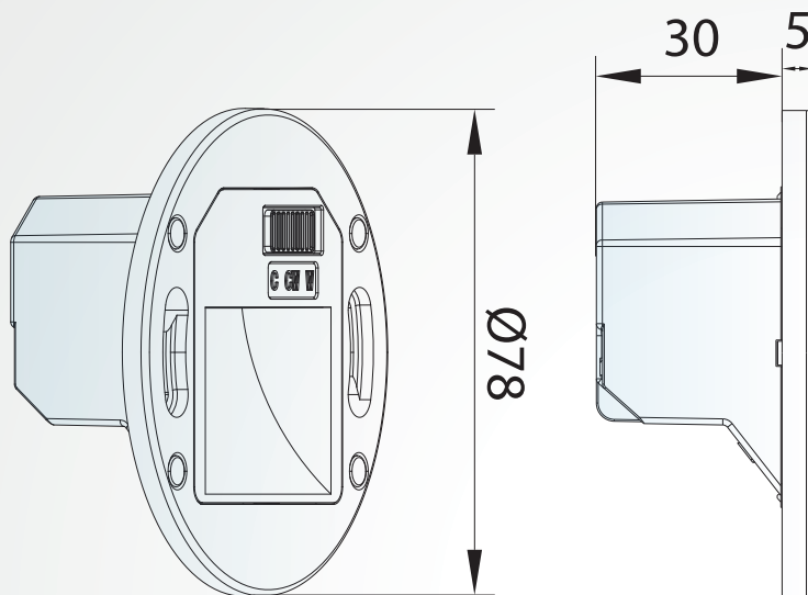
OST-001WH-CCT
